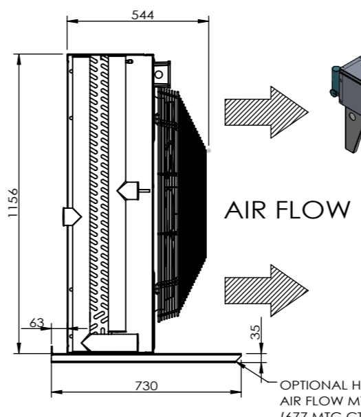
SIDE ELEVATION (OPTIONAL HORI. AIR FLOW)
