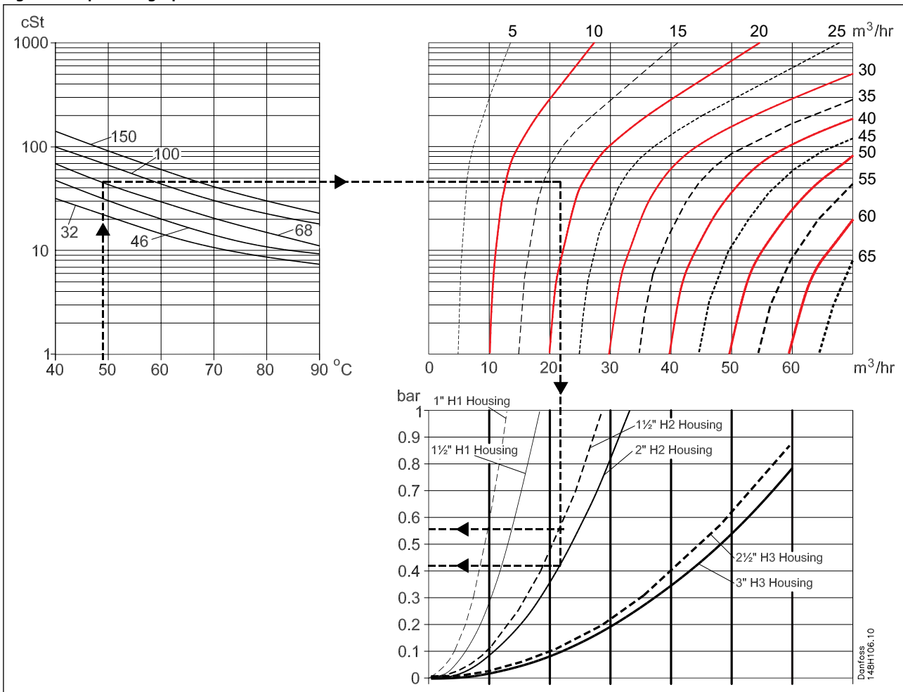
Figure 5: Capacities graphs
