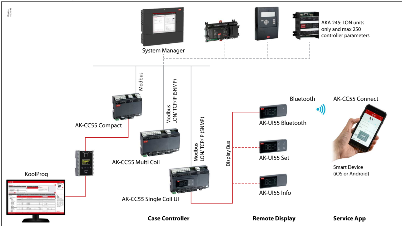
Figure 10: Connectivity
