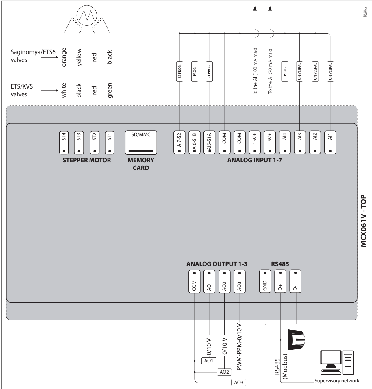
Figure 1: Top board
