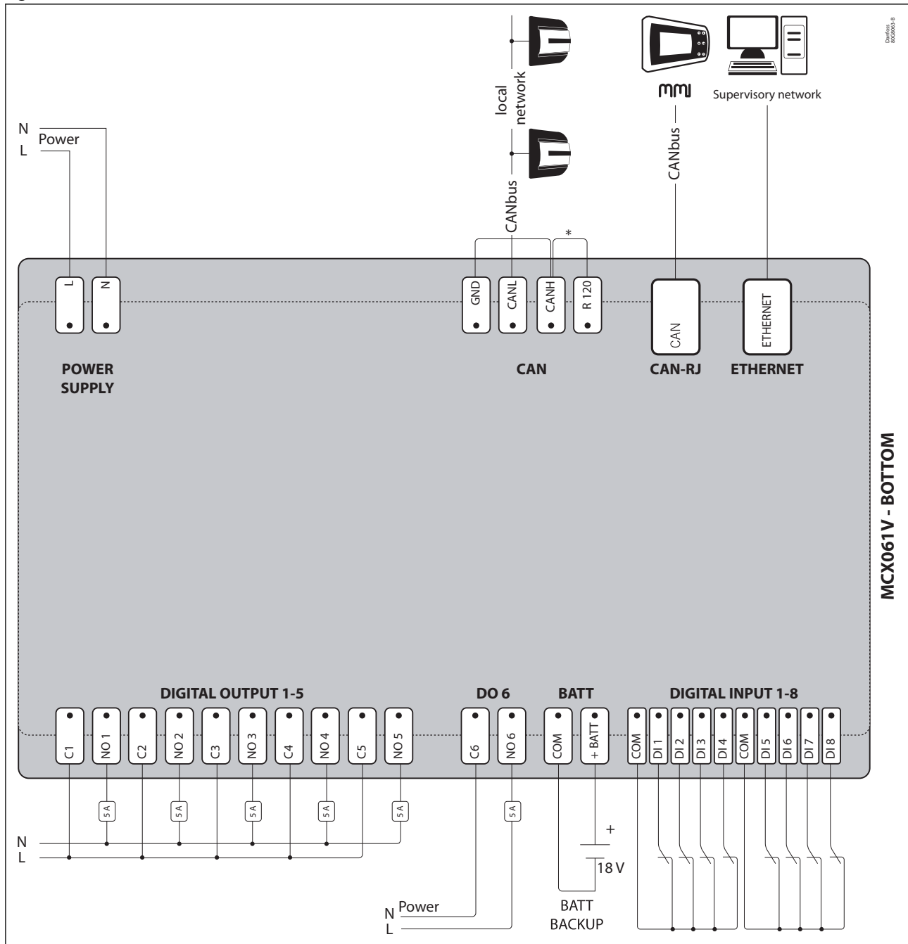
Figure 2: Bottom board
