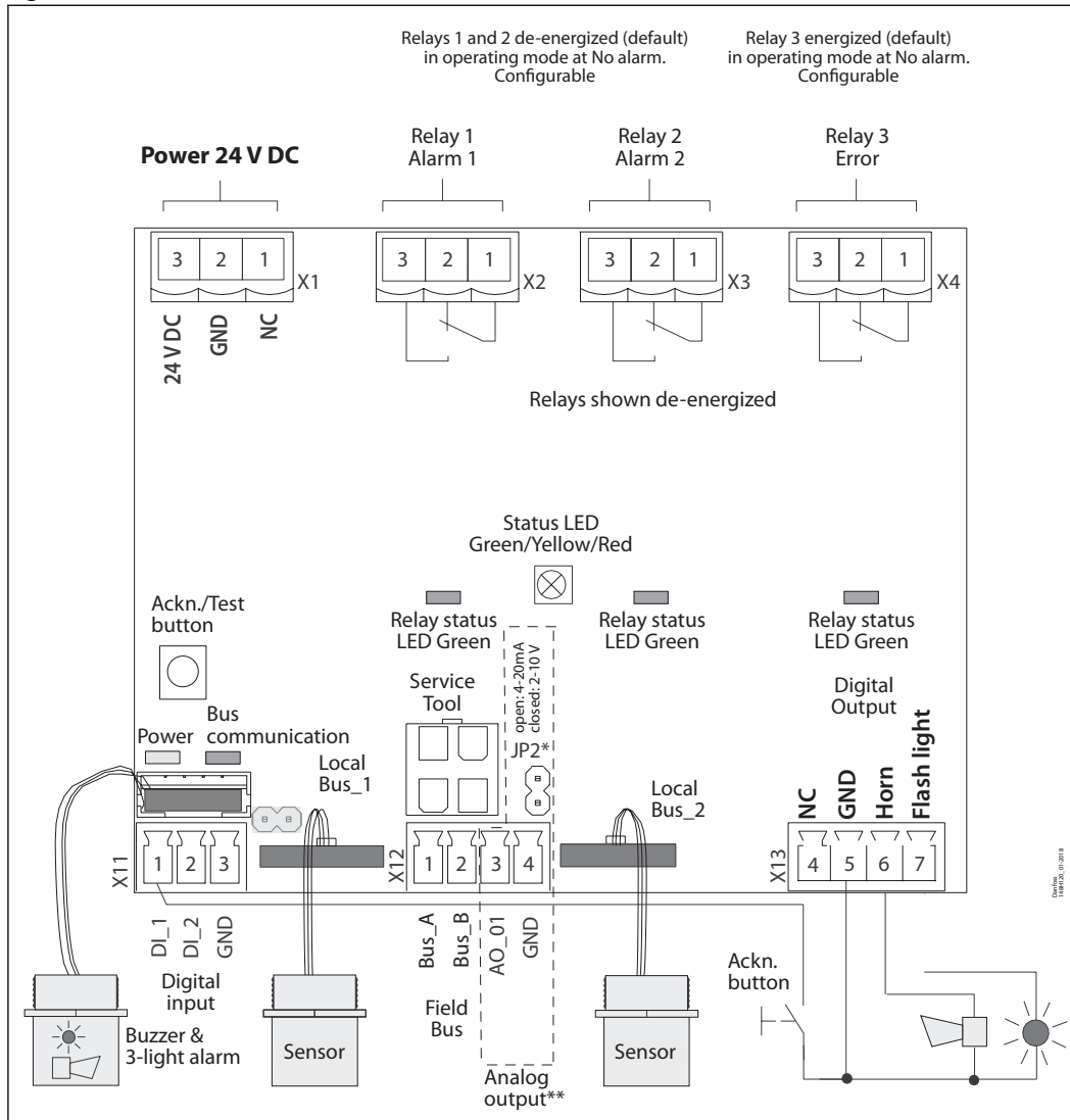
Figure 2: Electrical connection
