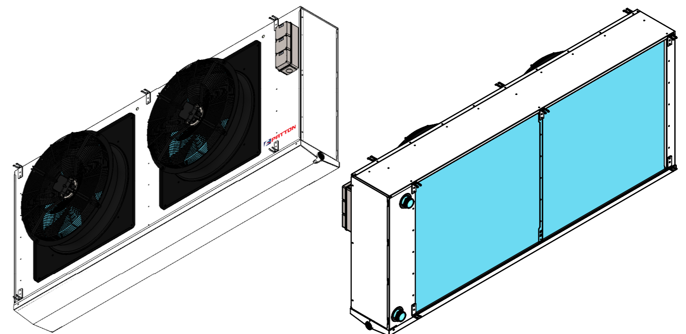
ISOMETRIC VIEWS (2 FAN)
