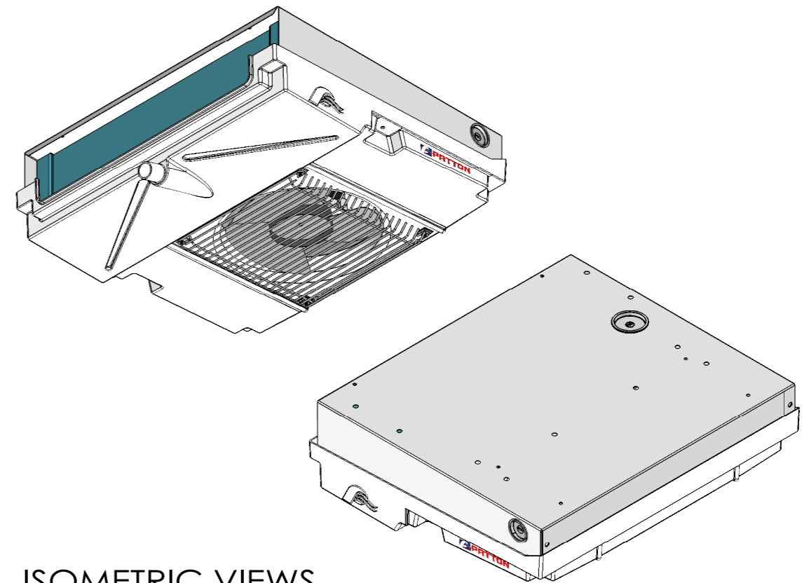
ISOMETRIC VIEWS
