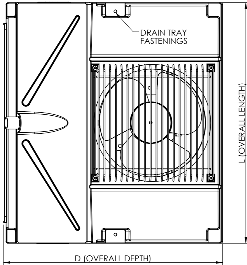
BOTTOM VIEW
