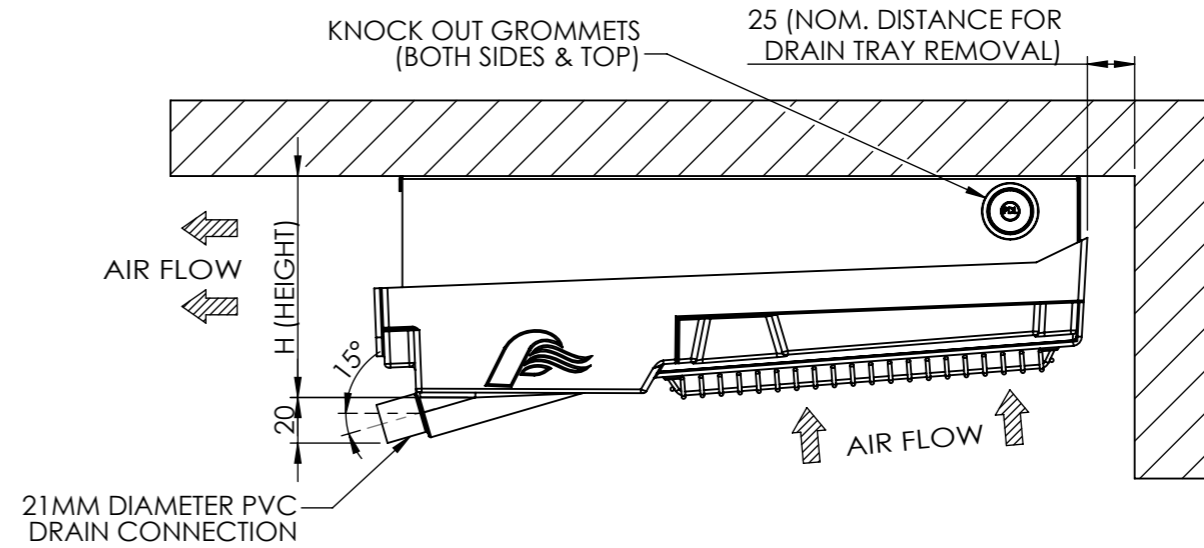
SIDE ELEVATION
